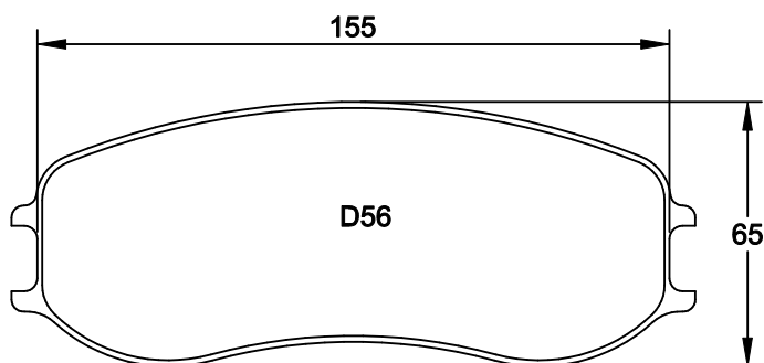
4920 = 22mm 4928 = 28mm Porsche 991 GT3 Cup front
