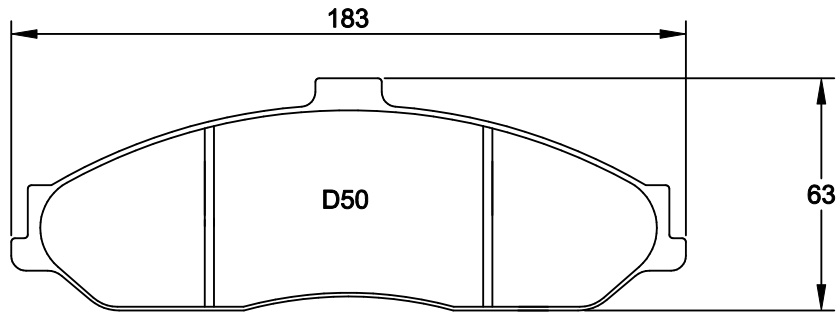
2213USA = 15mm Corvette C5, C6 base
