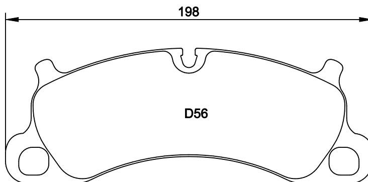
4921 = 20mm 4929 = 26mm Porsche 991 GT3 Cup rear
