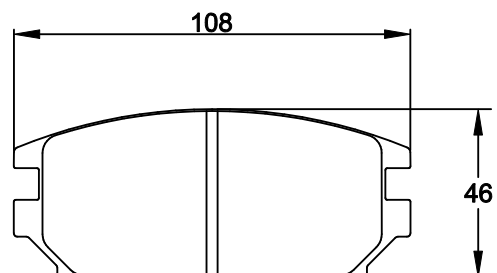
2445 = 15.5mm Mitsubishi rear
