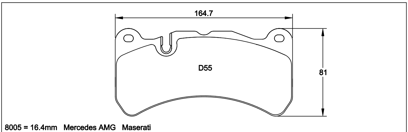
8003 = 17.5mm 8004 = 19.5mm Porsche
